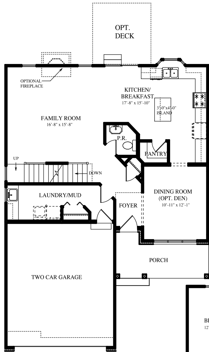
FIRST FLOOR PLAN 942 S.F.
