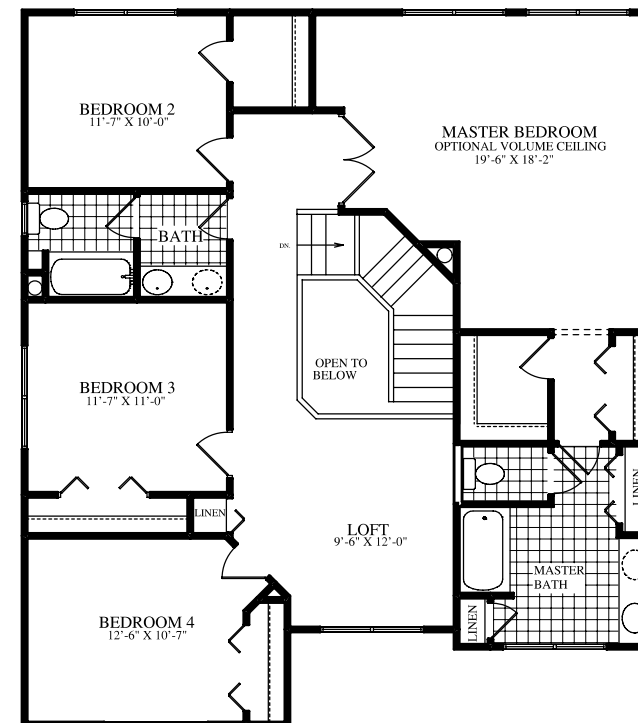
SECOND FLOOR PLAN 1314 S.F.
