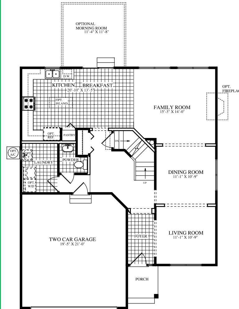
FIRST FLOOR PLAN 1100 S.F.
