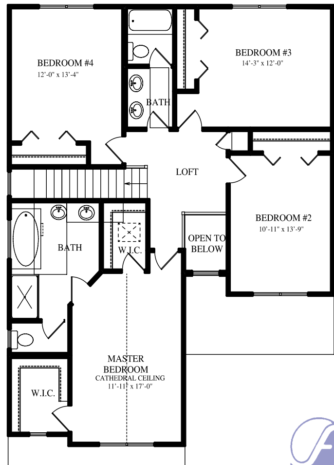
SECOND FLOOR PLAN 1,250 S.F.
